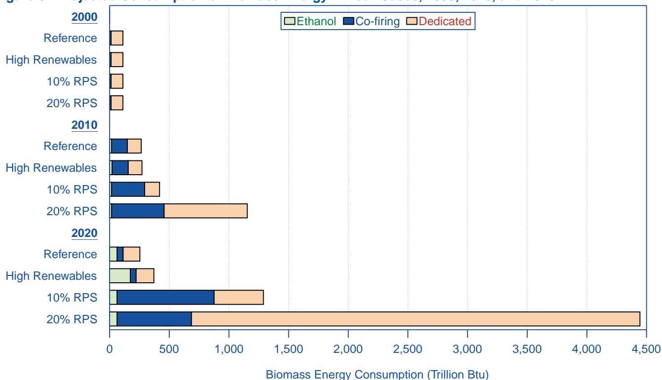
Figure 5. Projected Consumption of Biomass Energy in Four Cases, 2000, 2010, and 2020
