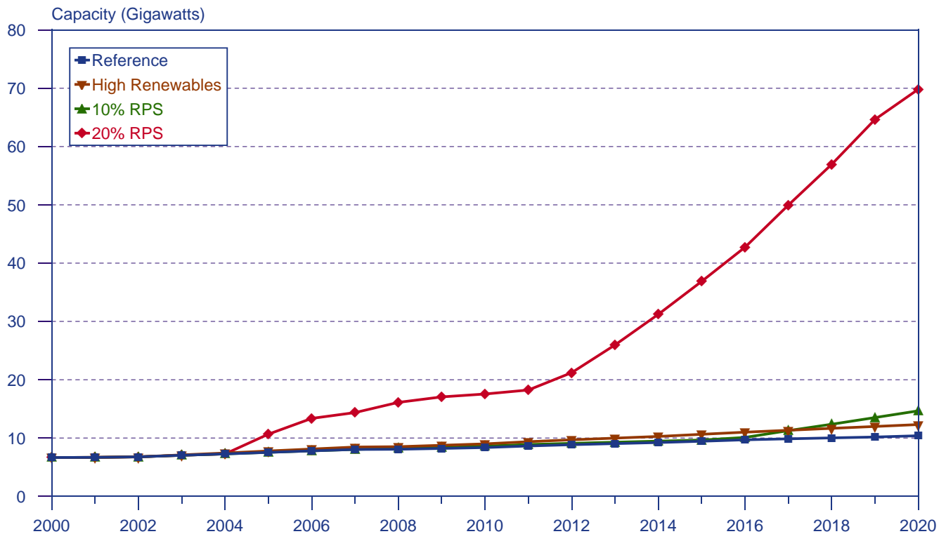
Figure 4. Projections of Biomass-Fired Generating Capacity in Four Cases, 2000-2020
