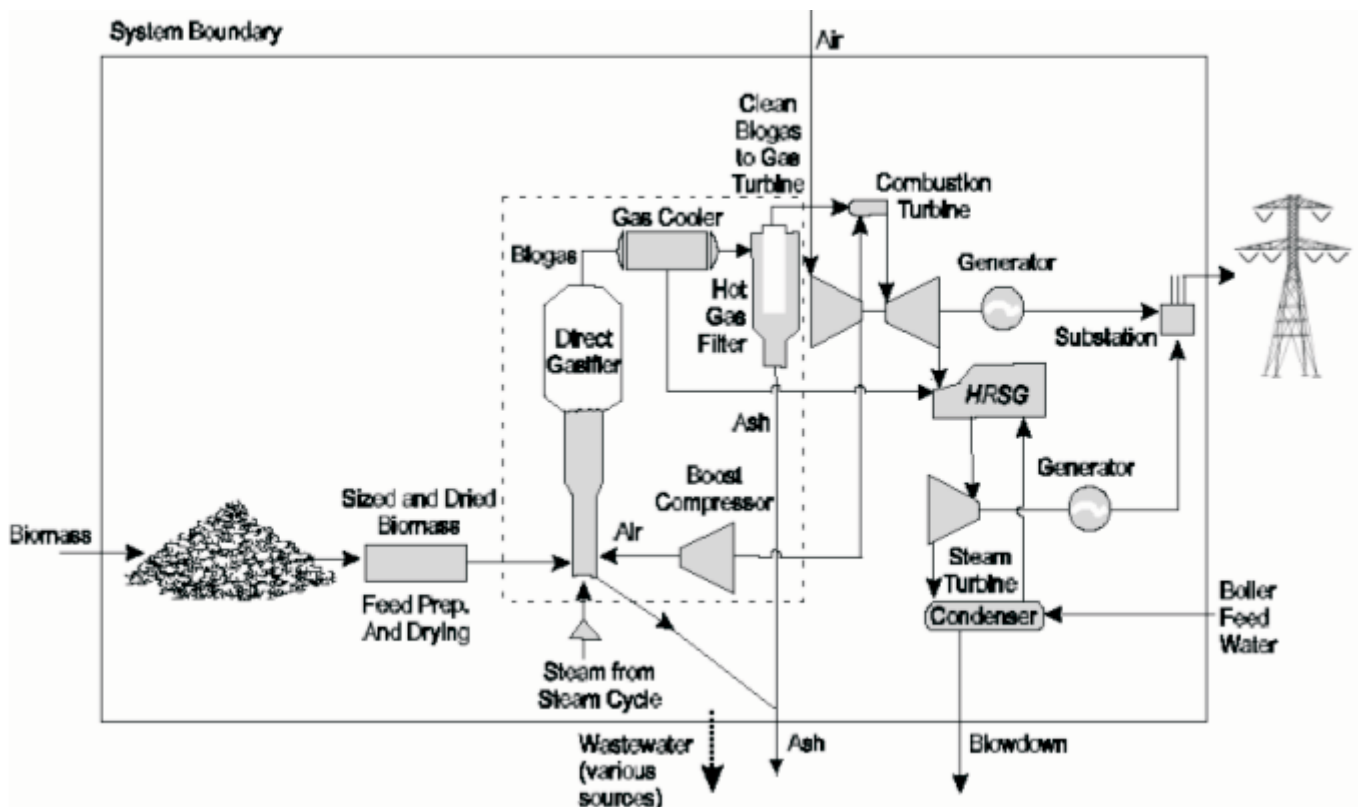
Figure 1. Biomass Integrated Gasification Combined-Cycle System Schematic
