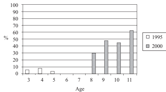
Fig. 2. Prevalence of myopia with age.
