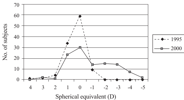
Fig. 1. Distribution of spherical equivalent refraction.
