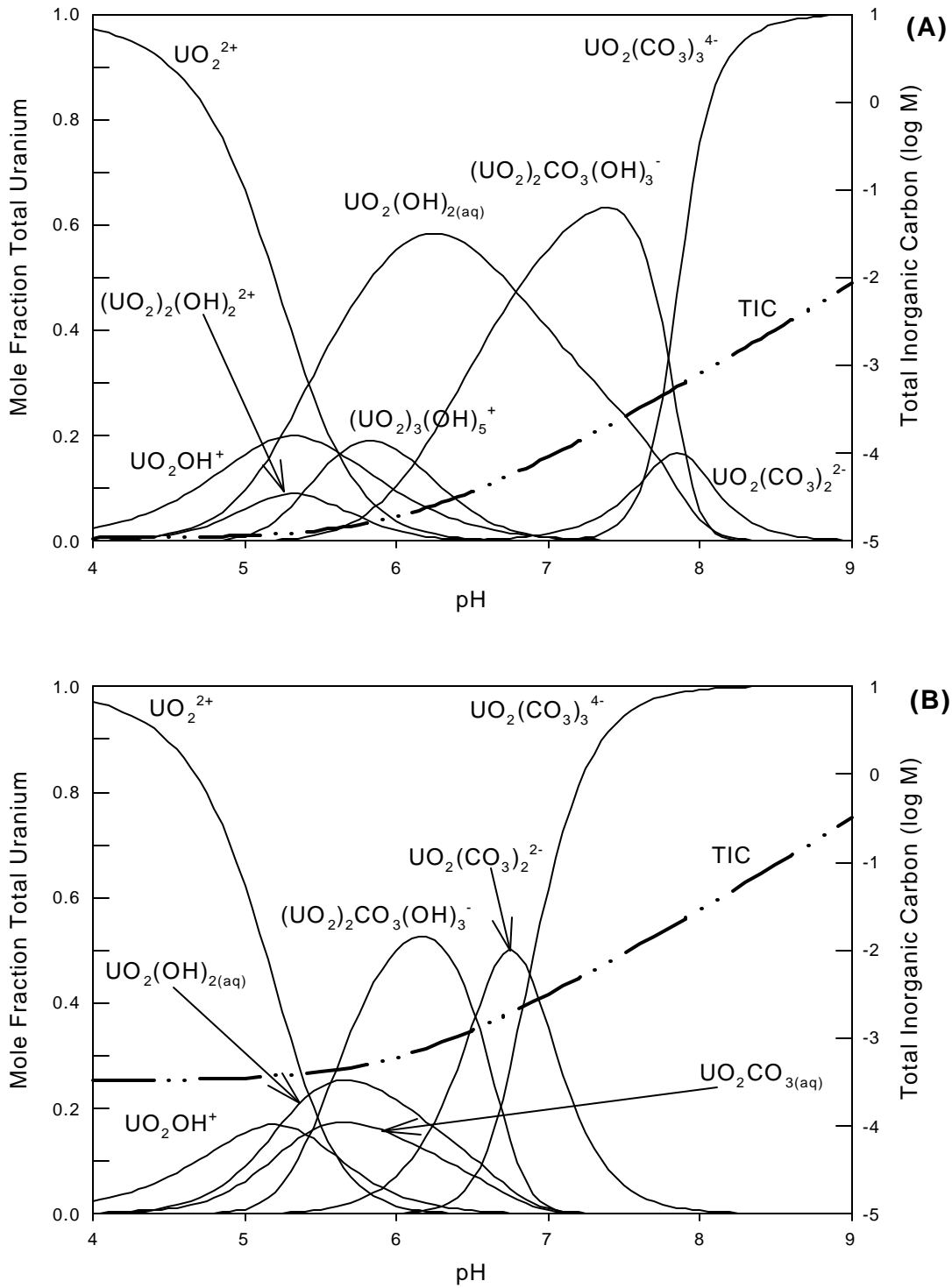
Fig.3.2. Uranium aqueous speciation as a function of pH considering both hydrolysis products and carbonate complexes. Species are plotted as mole fraction total uranium versus solution pH. U_{TOT} = 10^{-5} M; I = 0.2 ; (A) P_{CO_2} = 10^{-3.5} ; (B) P_{CO_2} = 10^{-2.0} ; no precipitation allowed.
