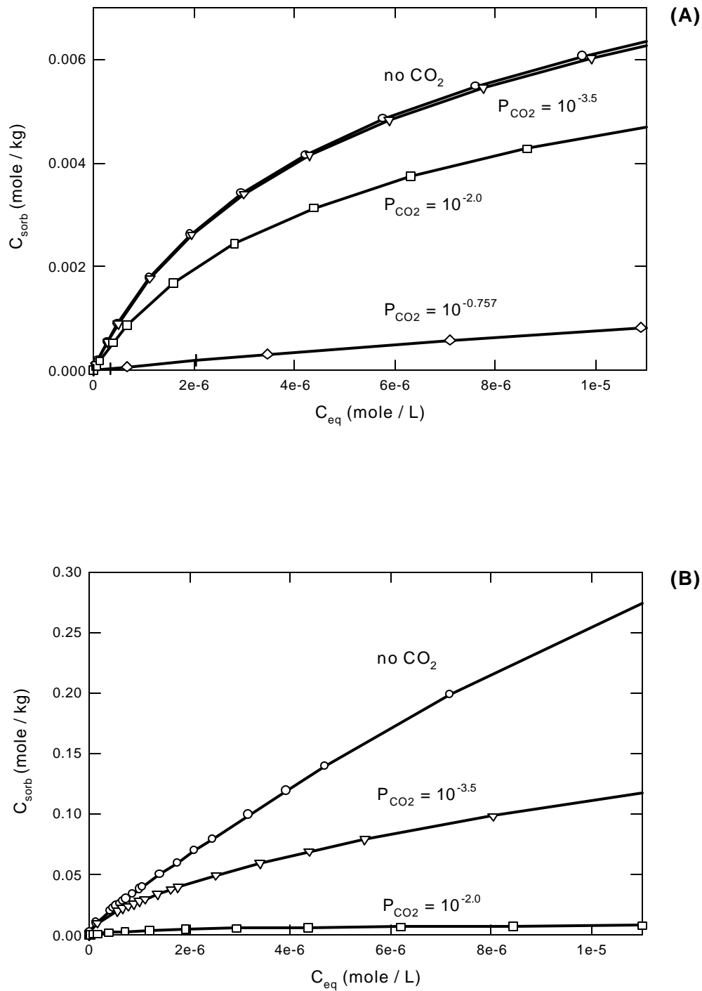
Fig. 3.6. Uranium sorption isotherms at different P_{\text{CO}_2} levels using a surface complexation model approach. Ionic strength = 0.2 M, (A) pH 5.5, and (B) pH 7.0. At pH 7 and P_{\text{CO}_2} = 10^{-0.757} there is no U sorption.
