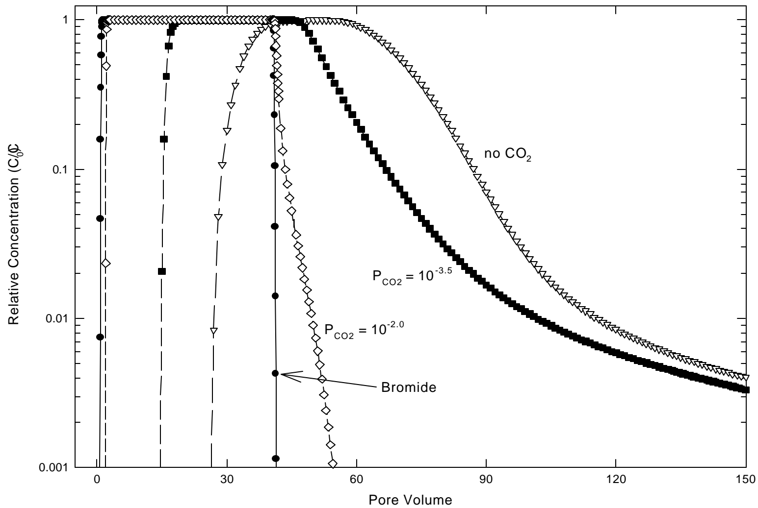
Fig. 3.7. Uranium breakthrough curves (relative concentration versus dimensionless time expressed as pore volumes) at different P_{CO_2} values. Bromide is included as representative of a nonreactive tracer. Note that the y-axis is log scale to illustrate tailing behavior. U_{TOT} = 10^{-5} M; pH = 7; I = 0.2 .
