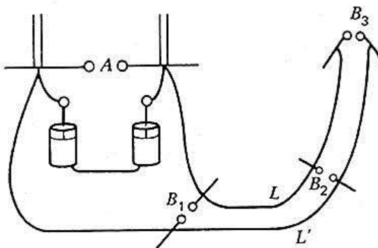
Fig. 2. While experimenting with this circuit, Oliver Lodge verified that the electromagnetic waves predicted by Maxwell do indeed exist.
