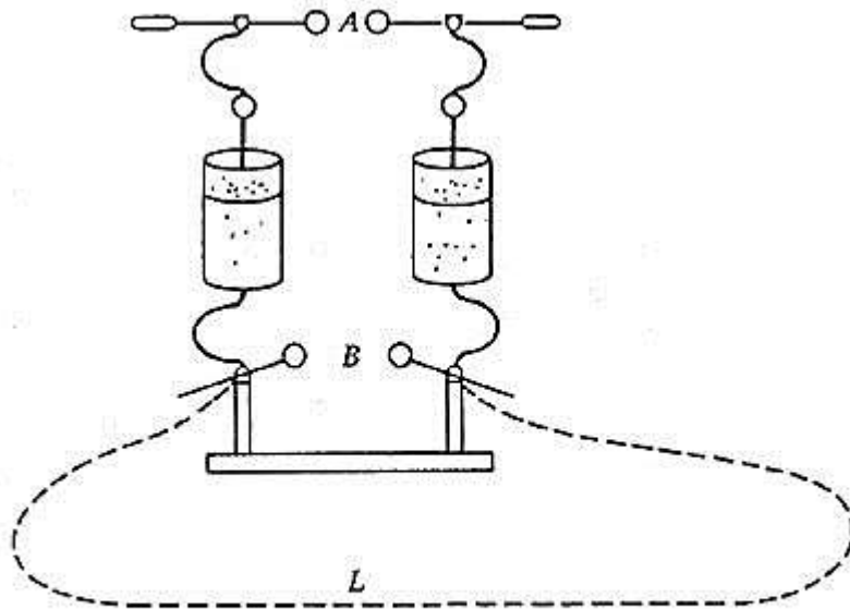
Fig. 1. Lodge's "alternate path" experiments demonstrated the effect of inductance in lightning protection circuits.
