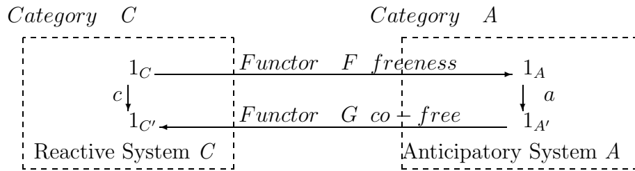
Fig. 1: Nature of Anticipatory Systems: a anticipates c
